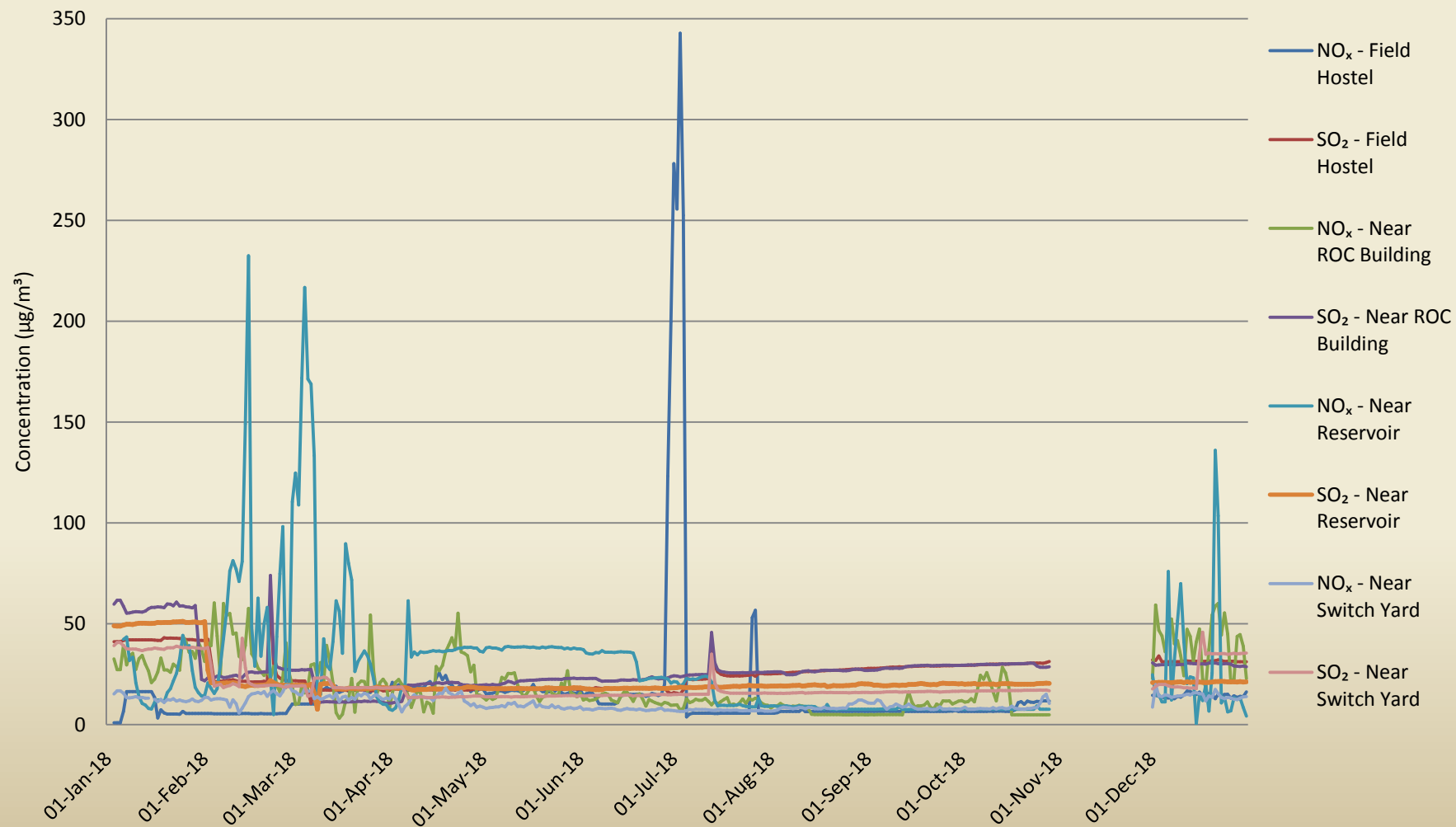
Annual Ambient Trend of Gaseous in M/s. M.B. Power (M.P.) Limited, Dist. Anuppur (M.P.)
